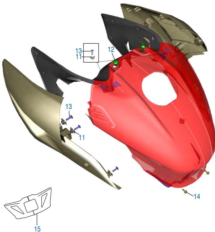
RH Mounting
